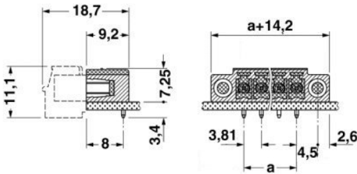
Dimensioned drawing
